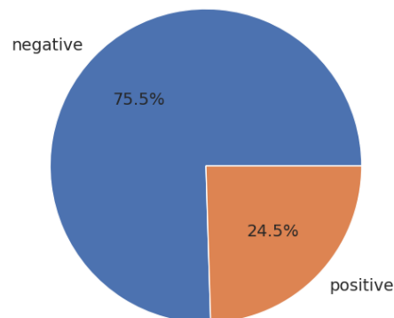
Figure 3. Sentiment Polarity
